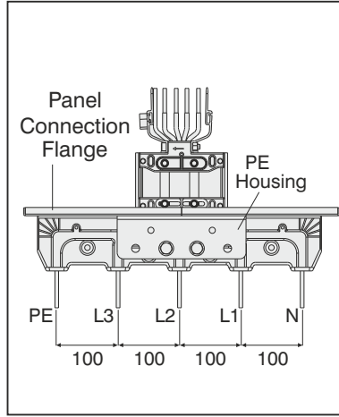
Opening on the panel board E-Line KX Panel Connection Busbar Flange
