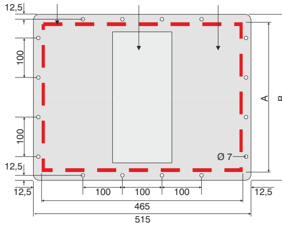
Opening on the panel board E-Line KX Panel Connection Busbar Flange
